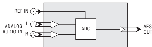
ASD-771p Functional Block Diagram
